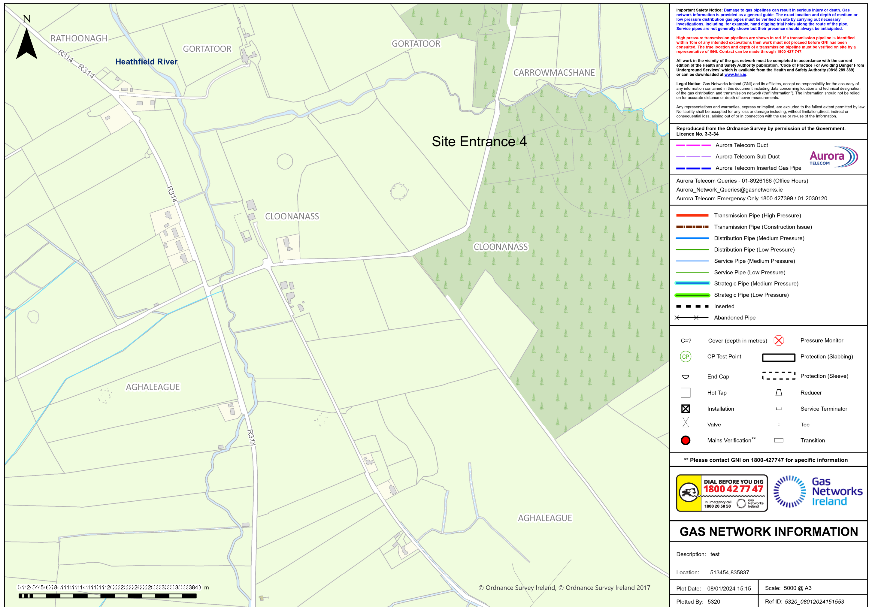
Figure 13.9 - Gas Network Information at Site Entrance 4
